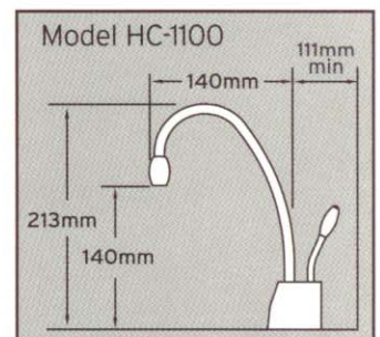
HC-1100 steaming hot or cold filtered water
